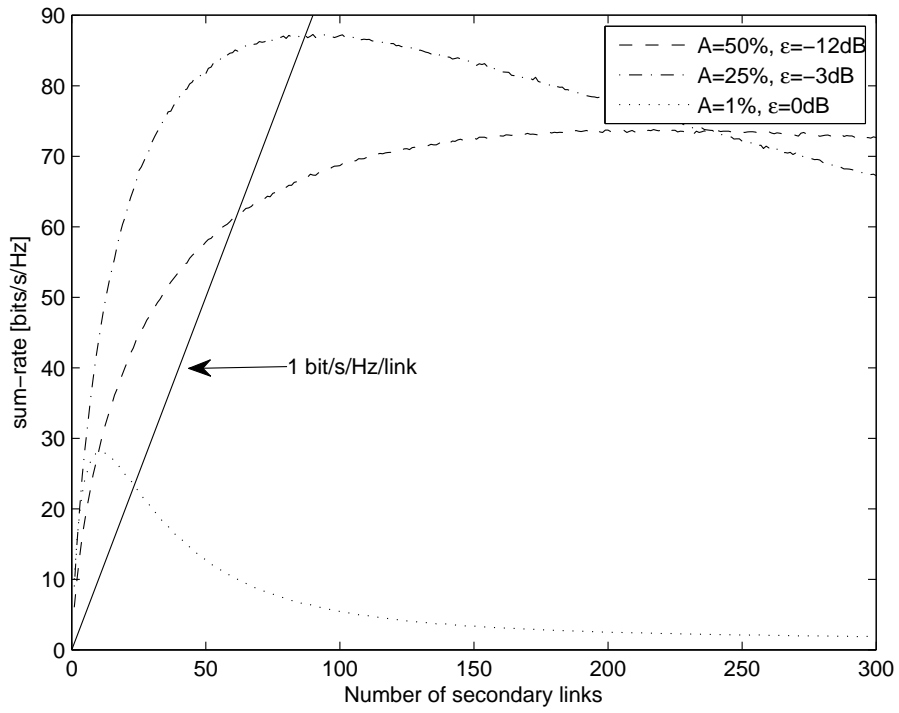
Figure 2: Total achievable sum-rate for the secondary system for d_0 = 0.1r , \alpha = 4 , \gamma = 6 dB, n = 21 .
