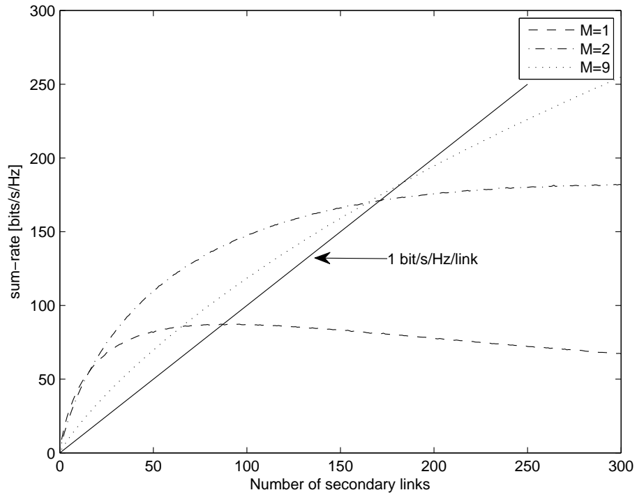
Figure 5: Comparison of the achievable sum-rate using time-division multiplexed repeater devices between the cognitive receiver and transmitter, for d_0 = 0.1r , \alpha = 4 , \gamma = 6 dB, n = 21 .
