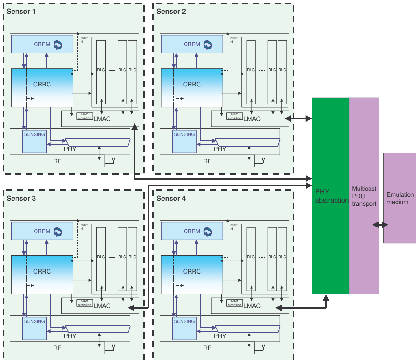
Figure 20: Demonstration scenario #1 implementation based on PHY emulation
