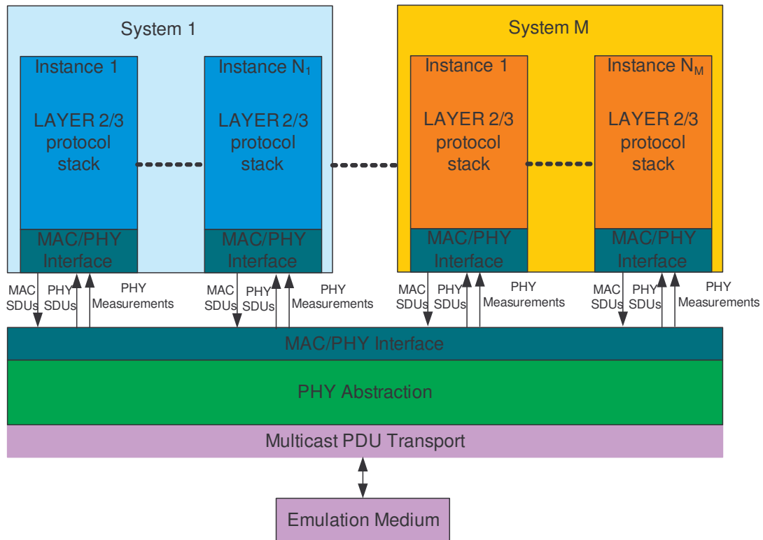
Figure 19: System architecture based on emulation environment
