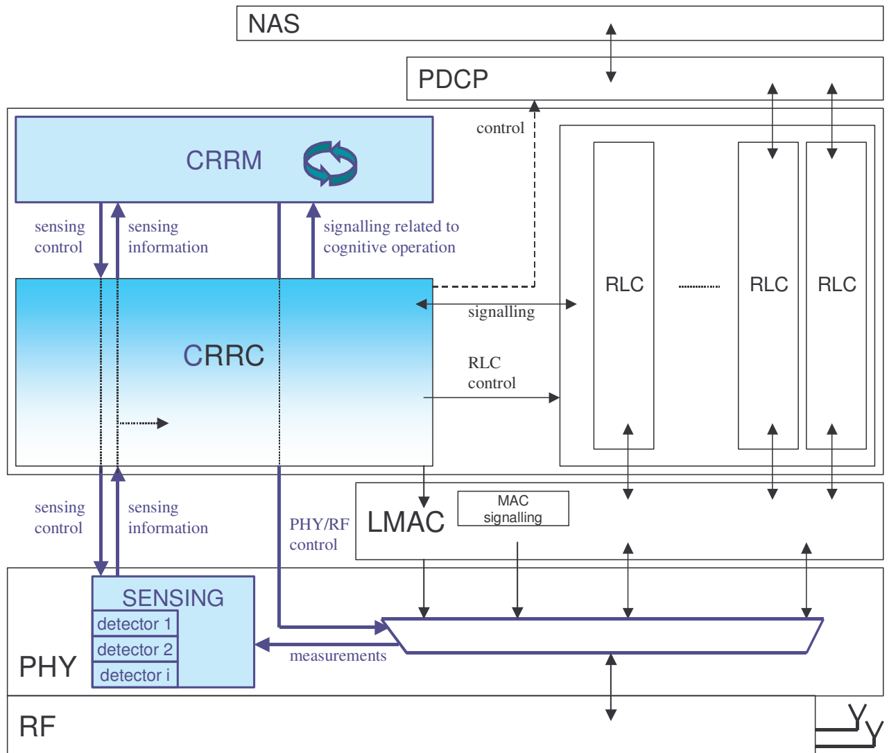
Figure 18: Protocol stack adaptation for demonstration scenarios implementation
