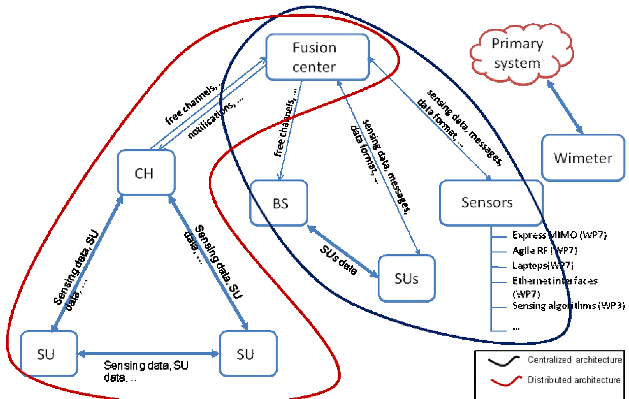
Figure 17: A schematic overview of the signalling messages needed for demonstration scenarios #1 and #2
